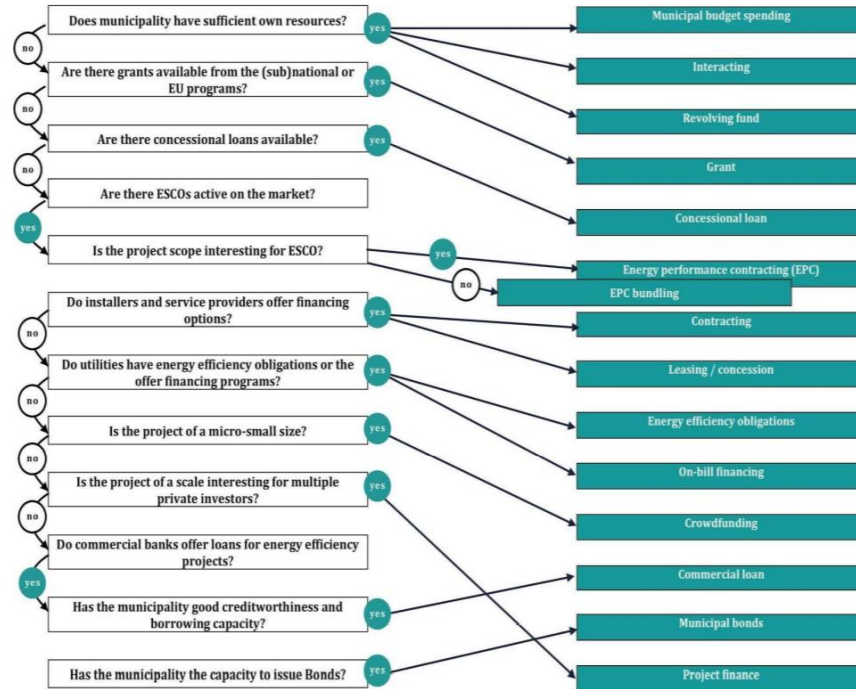
Figure 1: Decision Tree
